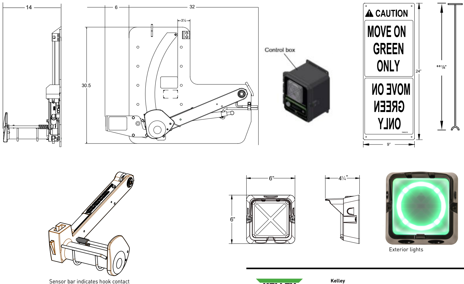
Sensor bar indicates hook contact
